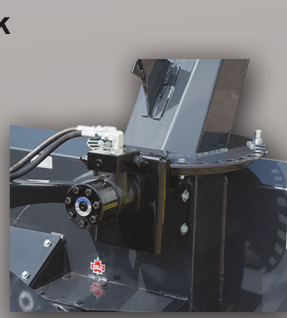
Hydraulic Rotation
