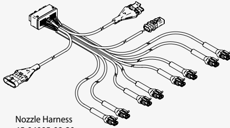
Nozzle Harness 45-04005-08-20
