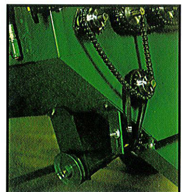
772 Screening Auger Drive
