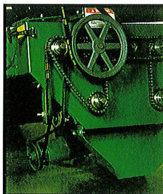
572 Screening Auger Drive
