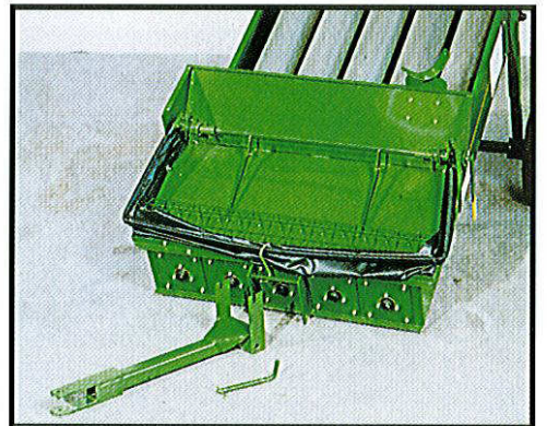
Patented Spring Loaded Collapsible Hopper and Standard Removable Hitch
