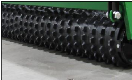
Nylon Corrugated Cultipacker Rings Optional Cast Iron
