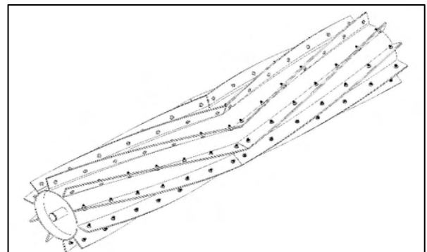
CB-Style Drum (Curved Blade) CB16A - 16" x 1/4" Wall - With Replacement Blades
