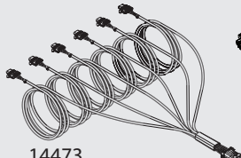
14473 Sensor Harness, 7'
