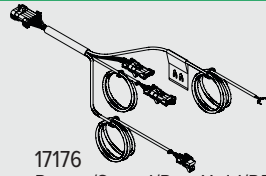
17176 Power/Speed/Run-Hold/RPM Harness, 10'
